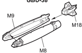
GBU-38
